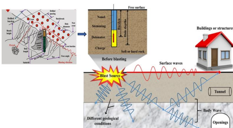
Figure 1. Propagation of ground vibration wave during rock blasting (Zhang et al., 2023)
